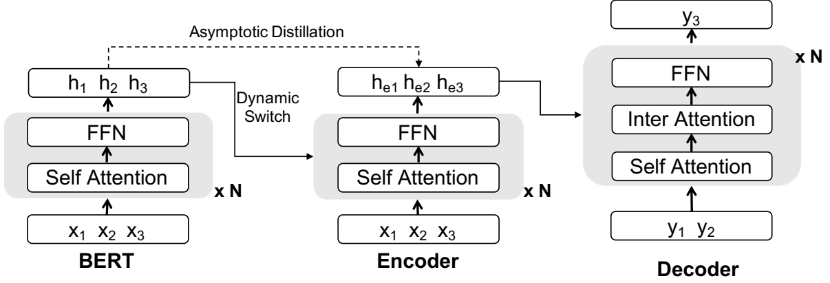
Figure 1: The overall CTNMT with asymptotic distillation and dynamic switch.
